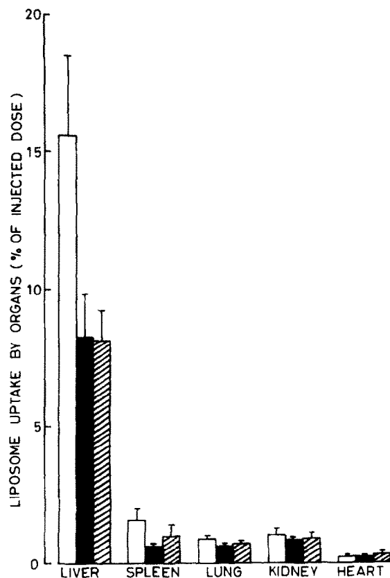
Fig.3. Distribution of egg [ ^{14}\text{C} ]PC containing liposomes in various organs at 3 h after the injection, before (open bars, ^{14}\text{C} ) and after coupling them to ^{125}\text{I} -labelled anti-rat erythrocyte F(ab') _2 (solid bars, ^{14}\text{C} ; shaded bars, ^{125}\text{I} ). Values shown are mean of 6 animals \pm SD.
