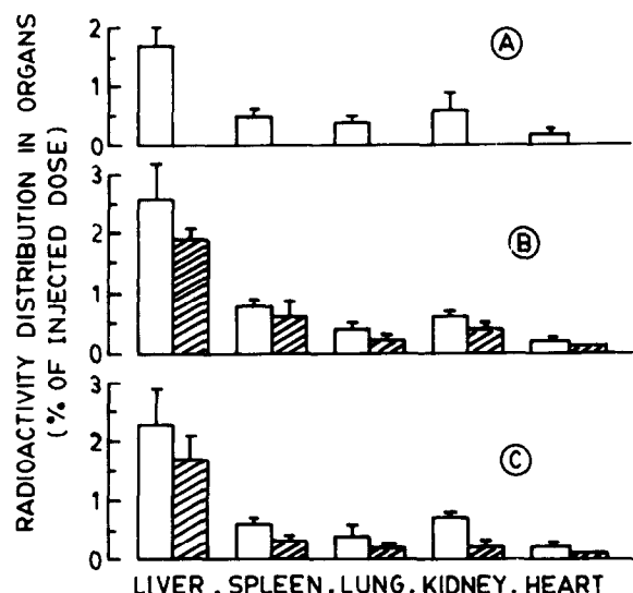
Fig.5. Distribution of radioactivity in various organs at 3 h after injecting ^{51}\text{Cr} -labelled liposome-treated (or untreated) red cells in rats. (A) Cells not treated with liposomes (open bars, ^{51}\text{Cr} ); (B) cells treated with egg [ ^{14}\text{C} ]PC-containing control liposomes (open bars, ^{51}\text{Cr} ; shaded bars, ^{14}\text{C} ); (C) cells treated with anti-rat erythrocyte \text{F(ab')}_2 bearing liposomes containing egg [ ^{14}\text{C} ]PC (open bars, ^{51}\text{Cr} ; shaded bars, ^{14}\text{C} ). Values are mean of 4 animals \pm SD.
