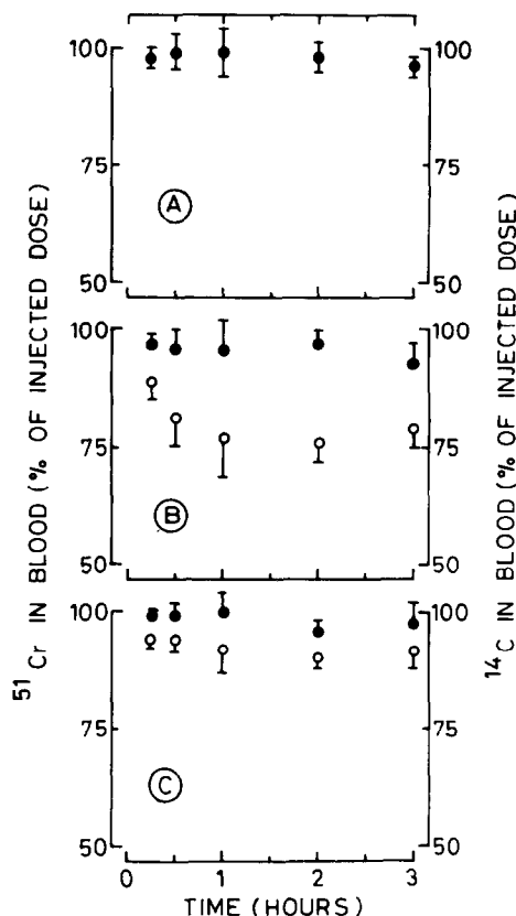
Fig.4. Survival of liposome-treated red cells in circulation of rats. (A) Cells not treated with liposomes (solid circles, 51 Cr); (B) cells treated with egg [ 14 C]PC-containing control liposomes (solid circles, 51 Cr; open circles, 14 C); (C) cells treated with anti-rat erythrocyte F(ab') 2 bearing liposomes containing egg [ 14 C]PC (solid circles, 51 Cr; open circles, 14 C). Values are mean of 4 animals ± SD.
