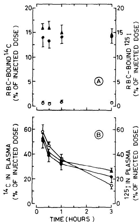
Fig.2. Liposomes containing egg [ ^{14}\text{C} ]PC were injected in rats (average weight 220 g) and the amount of radioactivity associated with erythrocytes (A) and the remaining radioactivity in plasma (B) at various periods of time determined, before (open circle, liposomal ^{14}\text{C} ) and after coupling them to ^{125}\text{I} -labelled anti-rat erythrocyte F(ab') _2 (solid circles, liposomal ^{14}\text{C} ; solid triangles, liposomal ^{125}\text{I} ), as in fig.1, except that 300 \mu\text{l} blood was drawn at each time point. Values shown are mean of 6 animals \pm SD.
